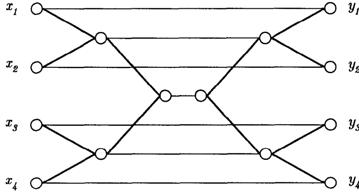
Figure 1: Data-flow for the prefix sum operation.
