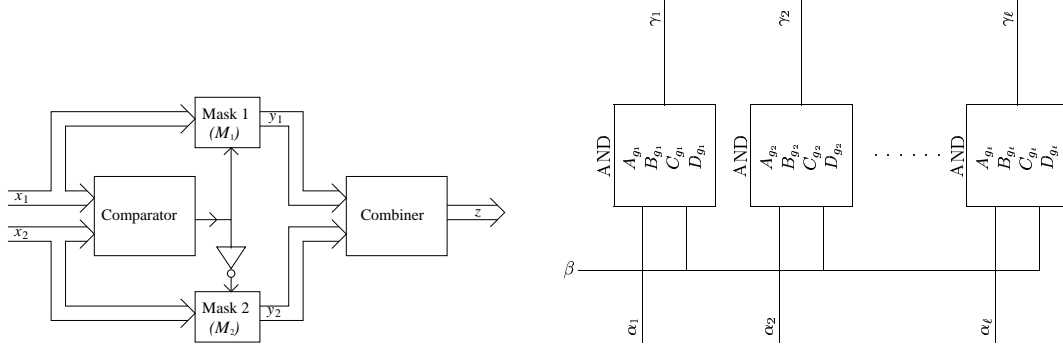
Figure 1: A circuit that computes z = \max(x_1, x_2) , along with the garbled subcircuit \mathcal{M}_2 . Wires \alpha_k get the input bits from x_2 , and output wires \gamma_k provide the bits of y_2 .
